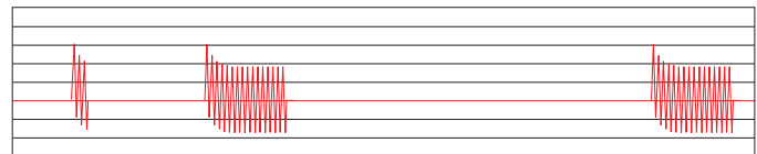
Current versus time—conventional recloser—fault from phase wire to grounded neutral
