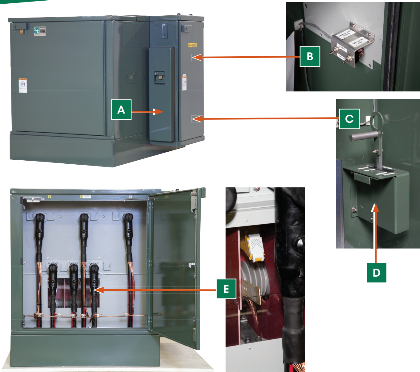
Figure 9. IntelliRupter fault interrupter accessories.
