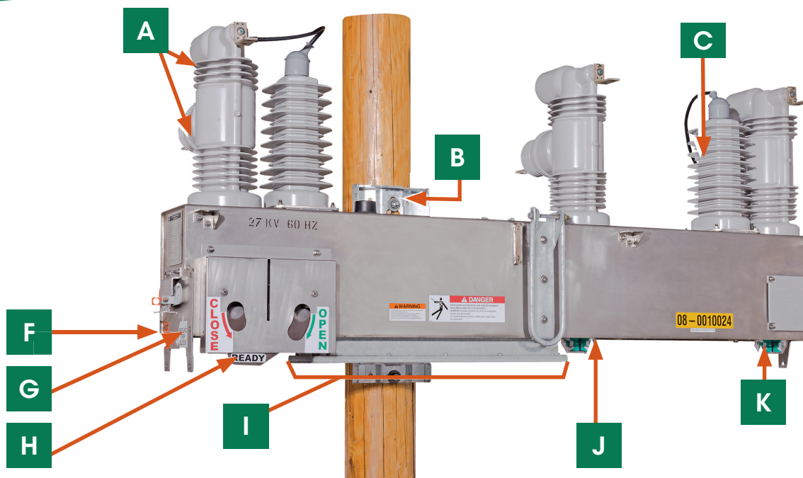
Figure 6. A Non-Disconnect Style IntelliRupter fault interrupter in an upright-crossarm mounting configuration, rated 15.5 kV maximum.
